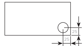
Typical Conduit Hole Location. Size = 25mm Conduit Knockouts
