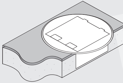
FFOB-145R Round Stainless Steel lid Bevelled Edge
