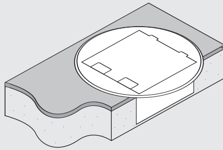
FFOB-148R Stainless Steel lid Bevelled Edge
