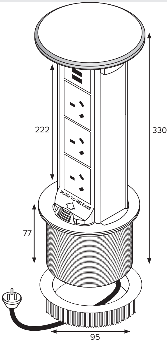
CDS3P2U Multiple Lid Colour Choices 3 x Square Autoswitched GPO 2 x USB Charge
