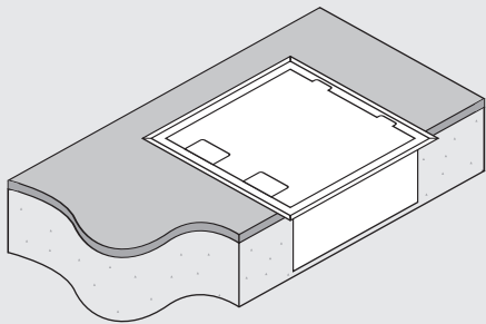
FFOB-245/8P8D Solid Stainless Steel lid
