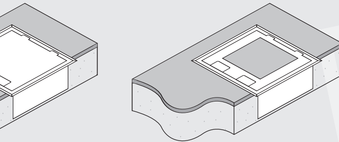
FFOB-248/8P8D Stainless Steel lid with 14mm Rebate
