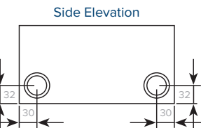
Typical Conduit Hole Location. Size = Combination 25mm/32mm Conduit Knockouts
